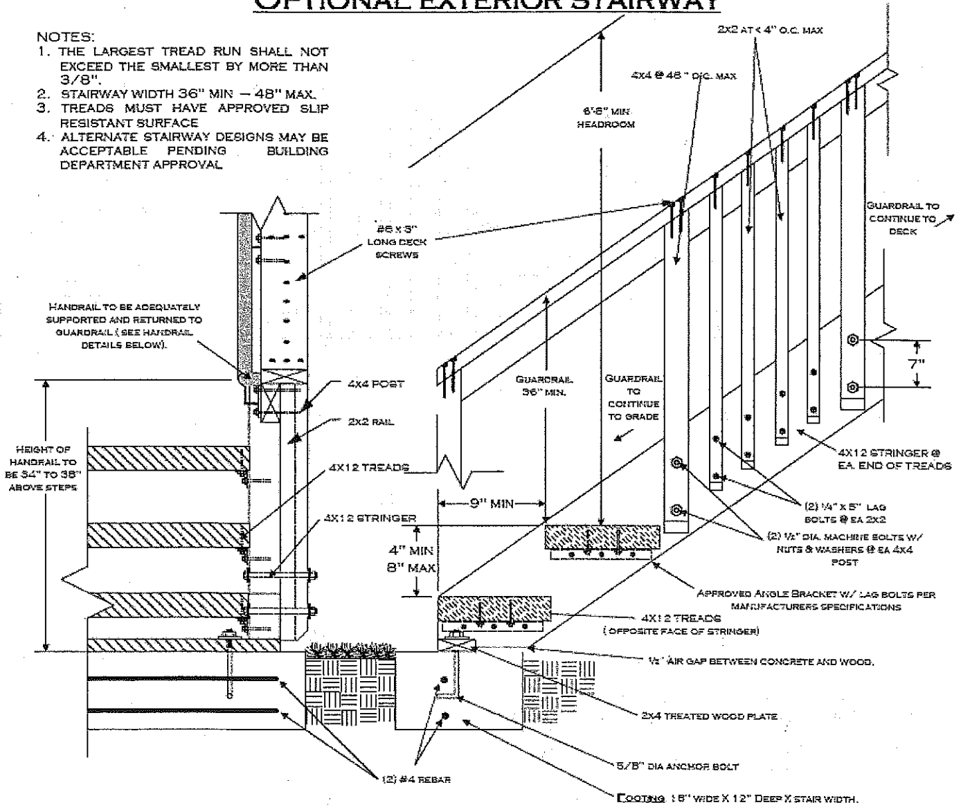
FRONT VIEW
