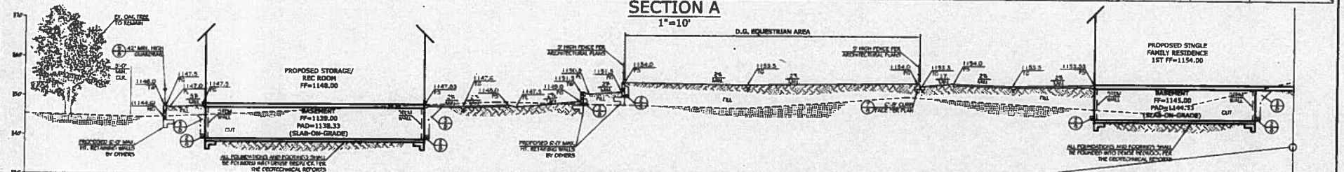
SECTION B 1"=10'
