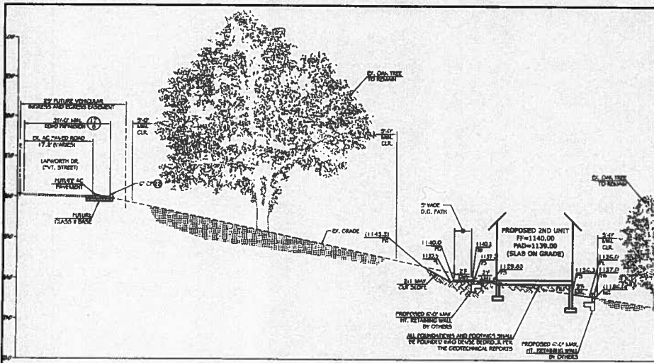
SECTION F 1"=10'
