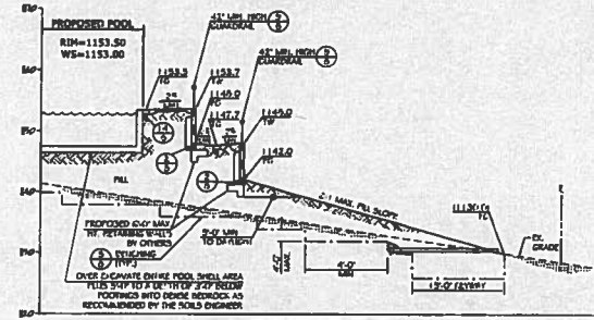
SECTION C 1"=10'
