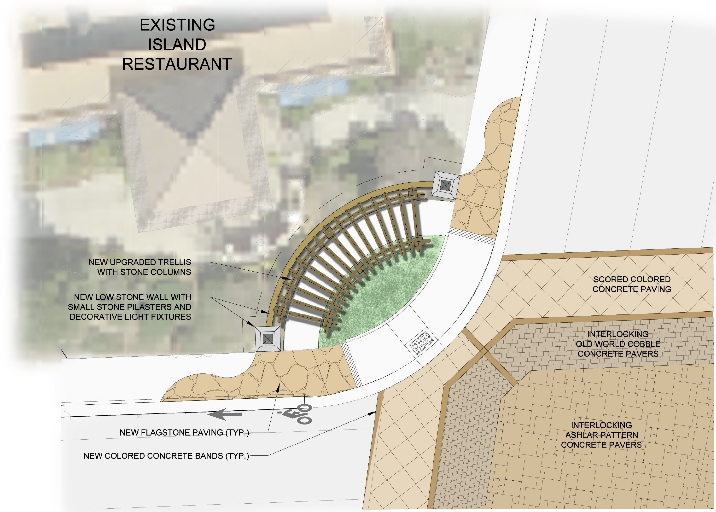
NORTHWEST CORNER PLAN SCALE : 1/8" = 1'-0"
