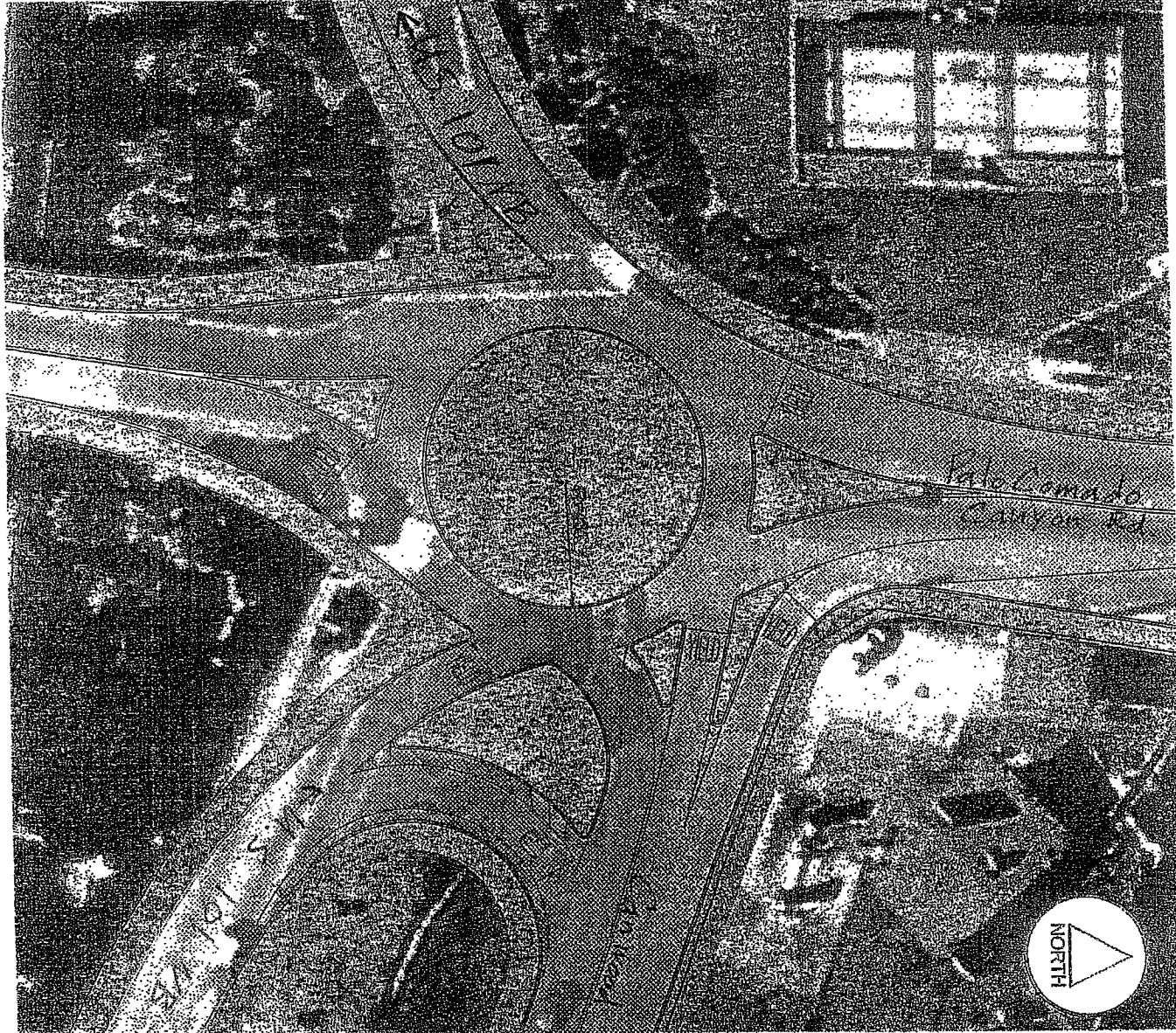
PALO COMADO CANYON RD/CANWOODST/U.S. 101 NB RAMPS ROUNDABOUT
